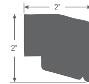
Large Sill Nose WPVCM-3591 1418311 - 16'
