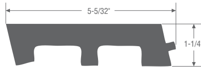
Replacement Sill 1 1/4" x 5 1/4" WPVCM-1005 1418301 - 12'
