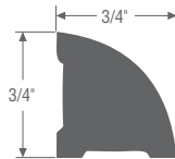
Quarter Round WPVCM-105 1202936 - 16'
