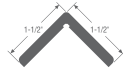
1 1/2" Outside Corner WPVCM-OSC 3112118 - 16'
