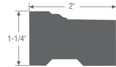
Brick Mould WPVCM-180 1202938 - 18'
