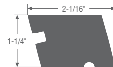
Window Sill Nose WPVCM-1006 1418302 - 12'
