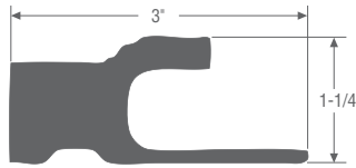
Brick Mould w/J-Channel and Fin WPVCM-180JF 1418300 - 18'
