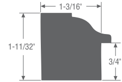
Back Band WPVCM-6931 1202943 - 16'
