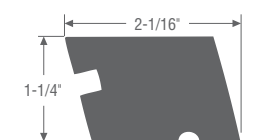
Window Sill Nose WPVCM-1006 1418302 - 12'
